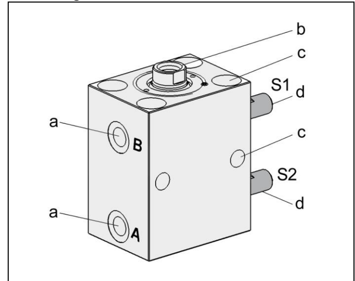
Fig. 1: components
