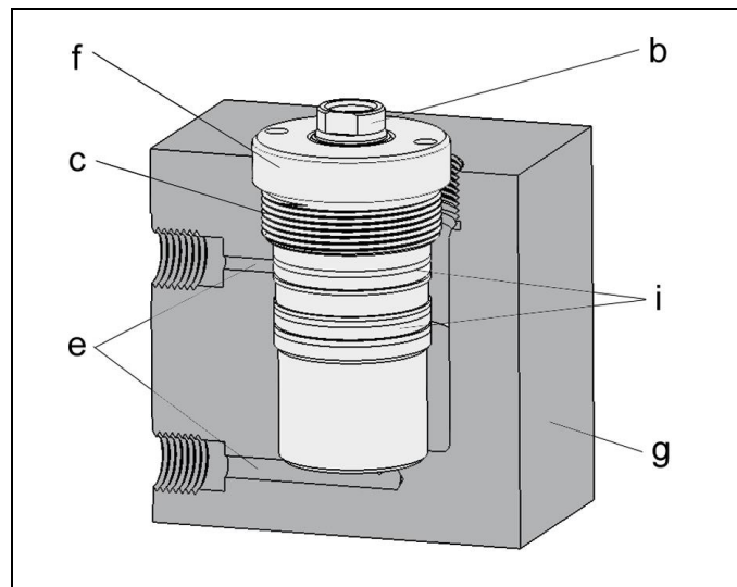
Fig. 1: Composants
