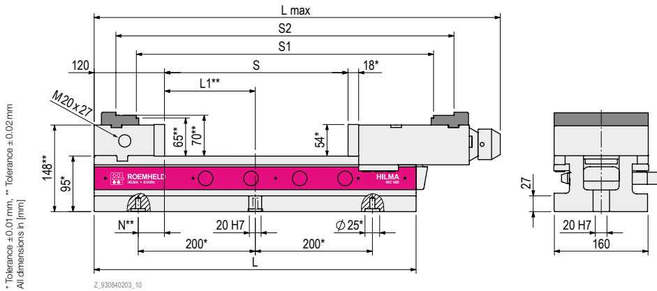
Figure: 930840203 Standard scope of supply Machine vise incl. crank handle and clamping jaws
