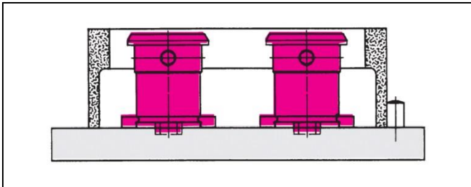
Figure 5: Mounting by segments
