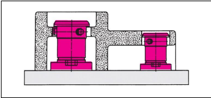
Figure 4: Flange mounting
