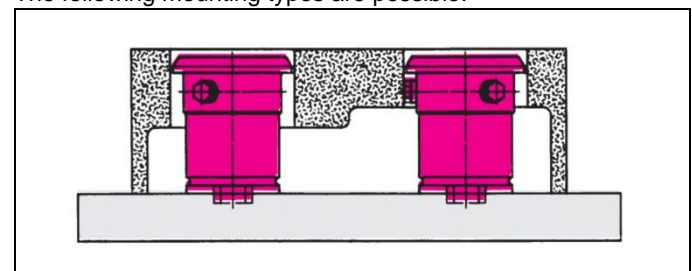
Figure 3: Direct mounting
