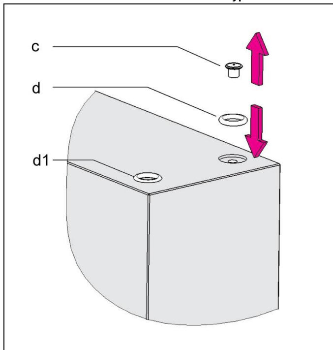
Figure 5: Example, preparation for hydraulic ports without pipes
