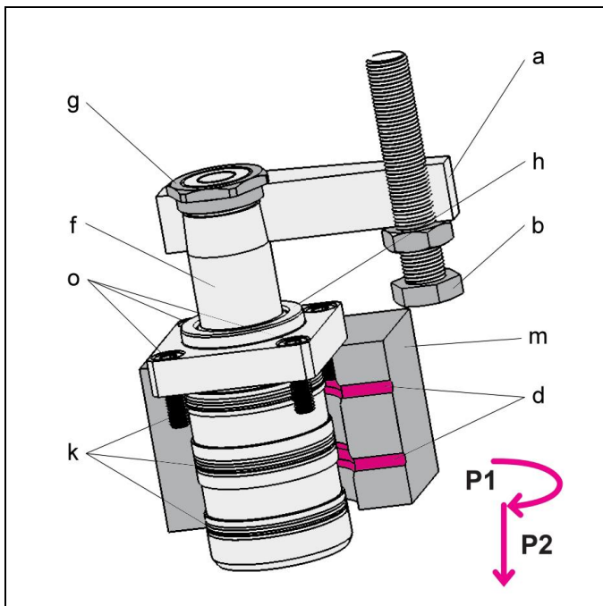
Figure 1: Components
