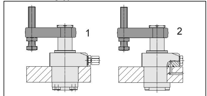
Figure 3: Mounting types
