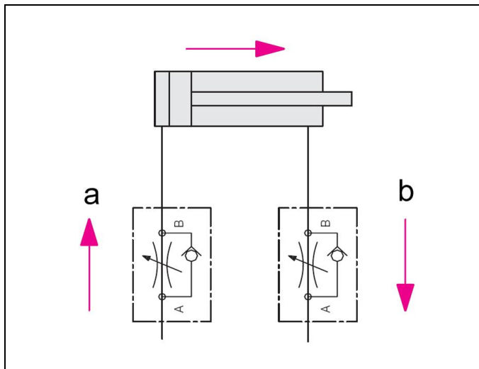
Figure 4: Hydraulic circuit diagram without flow control valves
