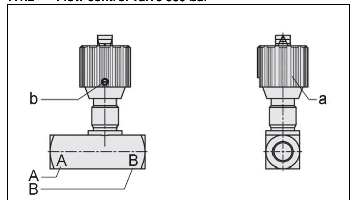
Figure 2: Flow control valve 350 bar
