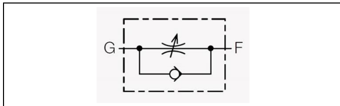
Figure 6: Flow control valve 500 bar
