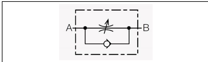
Figure 5: Flow control valve 350 bar
