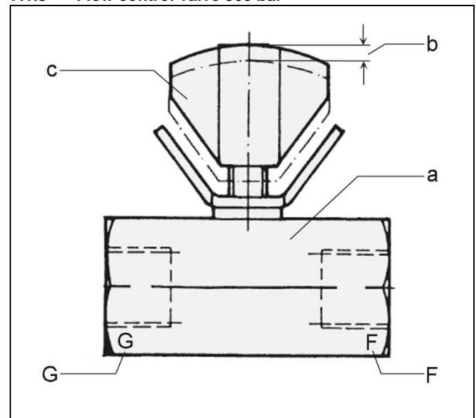
Figure 3: Flow control valve 500 bar
