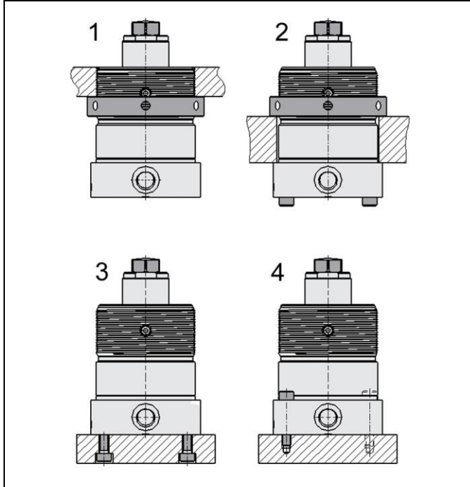
Figure 2: Fixing possibilities
