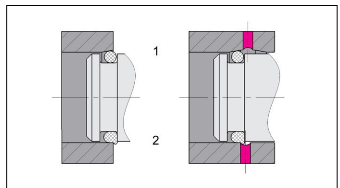
Figure 4: Installation with insertion chamfer and cross hole
