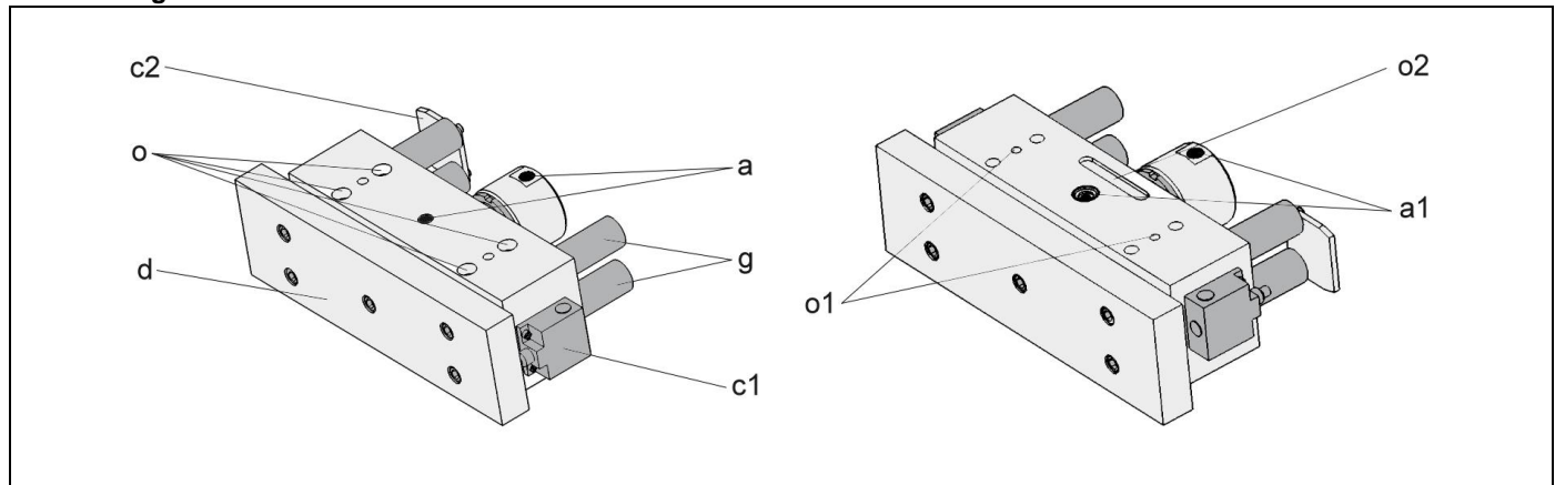
Figure 1: Components, optionally supplied with two mechanical limit switches
