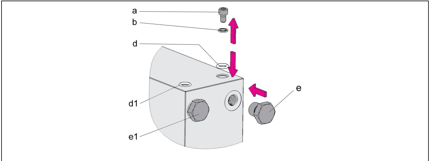
Figure 3: Example of the preparation for hydraulic ports without pipes
