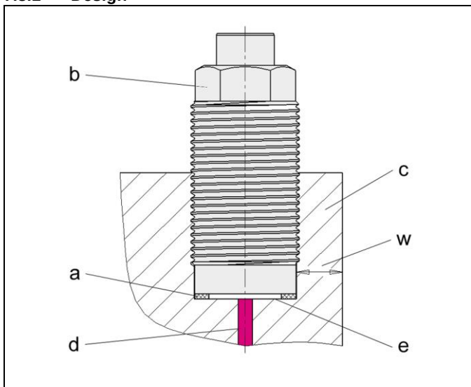
Figure 3: Mounting of the axial seal at the plane surface
