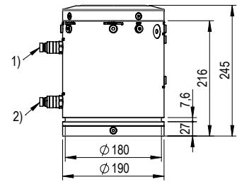
1) STARK.balance.3 release connection 2) STARK.classic.3 release connection
