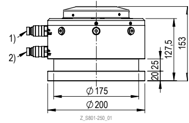
1) STARK.balance.2 release connection 2) STARK.classic.2 release connection
