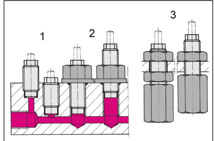
Figure 2: Fixing possibilities
