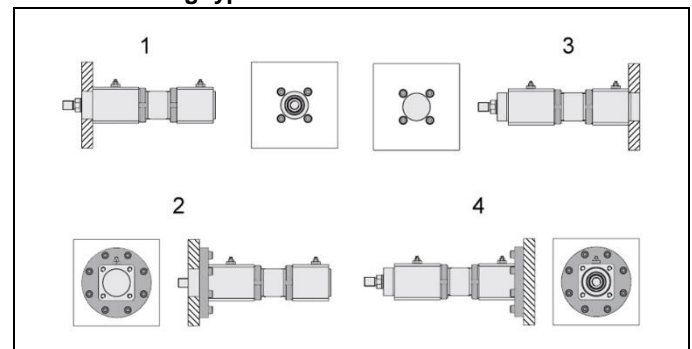
Figure 2: Fixing possibilities
