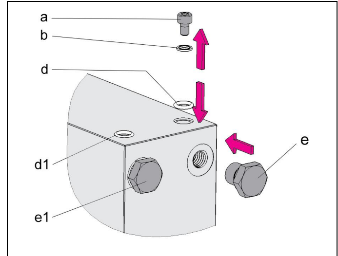
Figure 5: Example of the preparation for hydraulic ports without pipes
