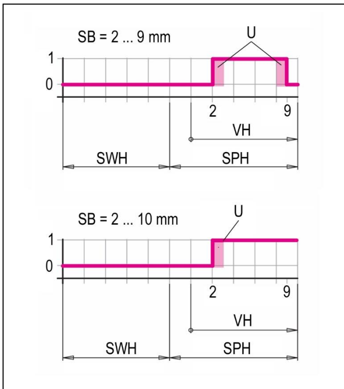
Figure 12: Signal course
