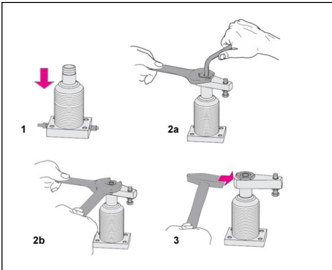
Figure 7: Assembly / disassembly (example)
