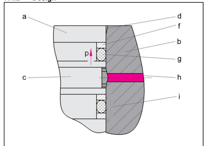
Figure 5: Components
