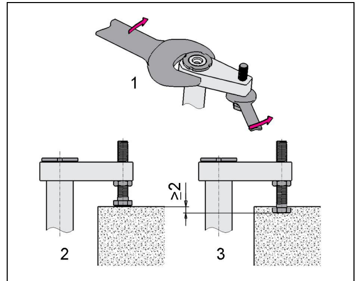
Figure 8: Adjustment of the clamping arm (example)
