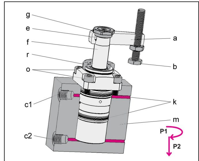
Figure 2: Components
