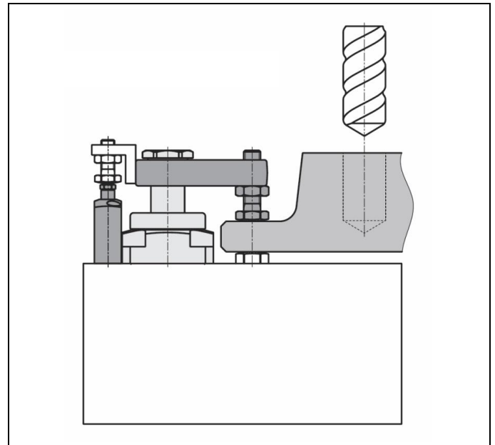
Figure 10: Application example
