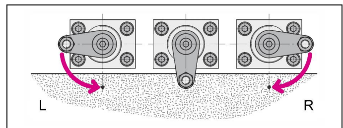
Figure 3: Swing direction
