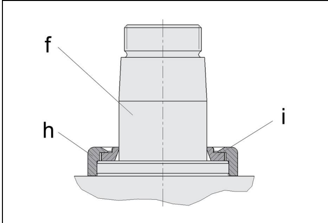
Figure 9: Metallic wiper
