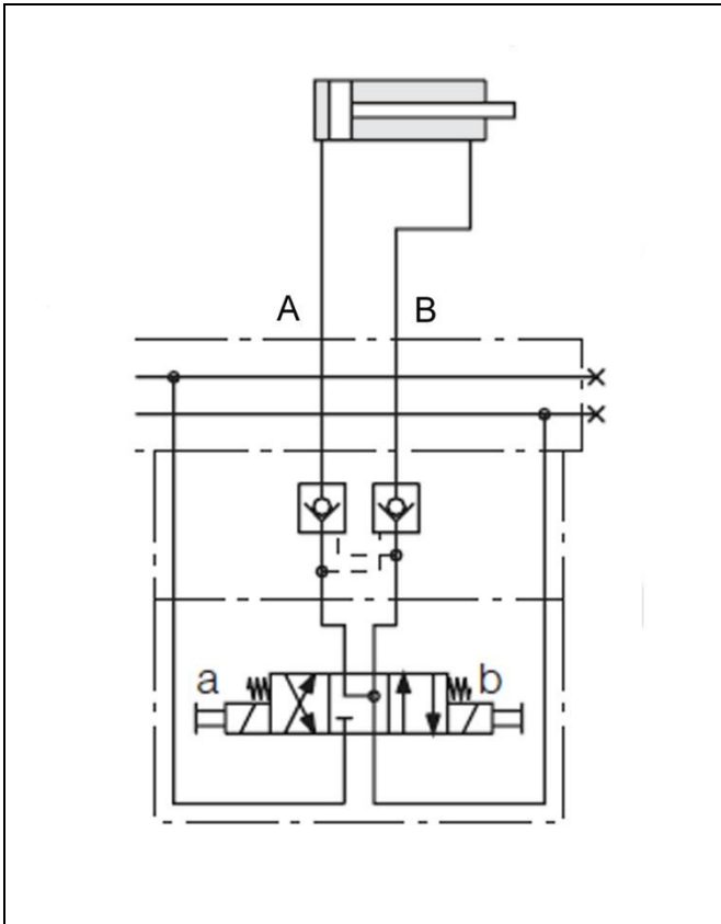
Figure 6: Presentation in the hydraulic circuit diagram
