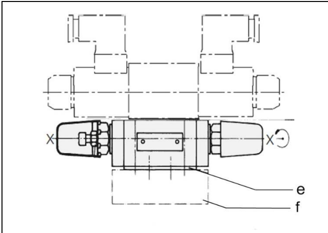
Figure 3: Twin flow control non-return valve
