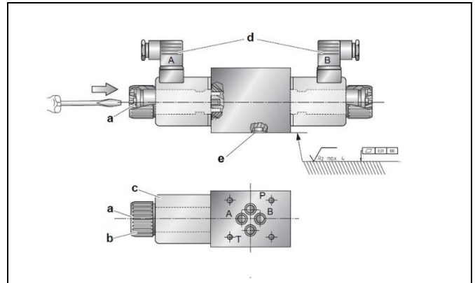
Figure 1: Design
