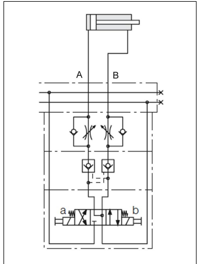
Figure 7: Presentation in the hydraulic circuit diagram
