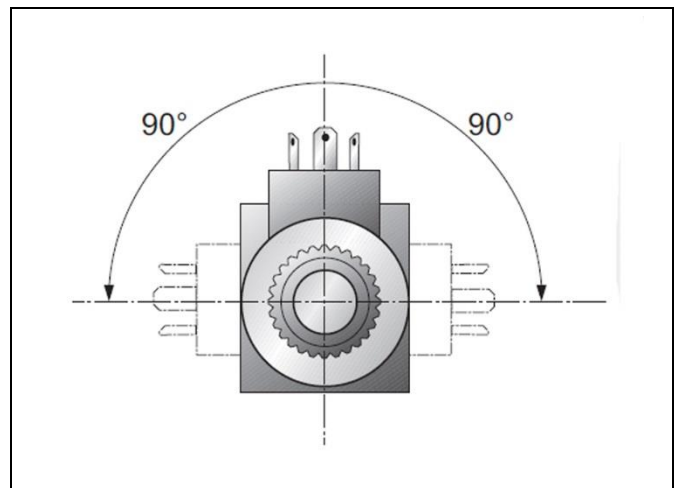
Figure 2: Solenoids
