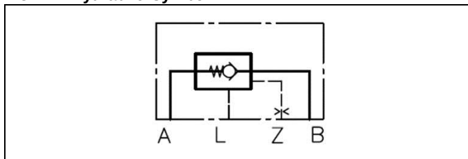
Figure 3: Presentation in the hydraulic circuit diagram
