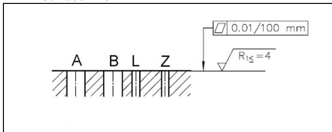
Figure 2: Surface finish
