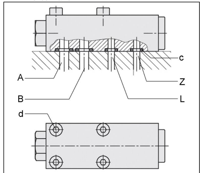
Figure 1: Manifold-mounting type
