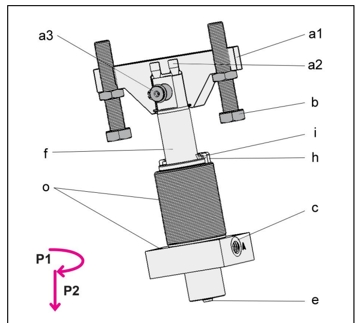
Figure 1: Components, pendulum eye (max . 500 bar)
