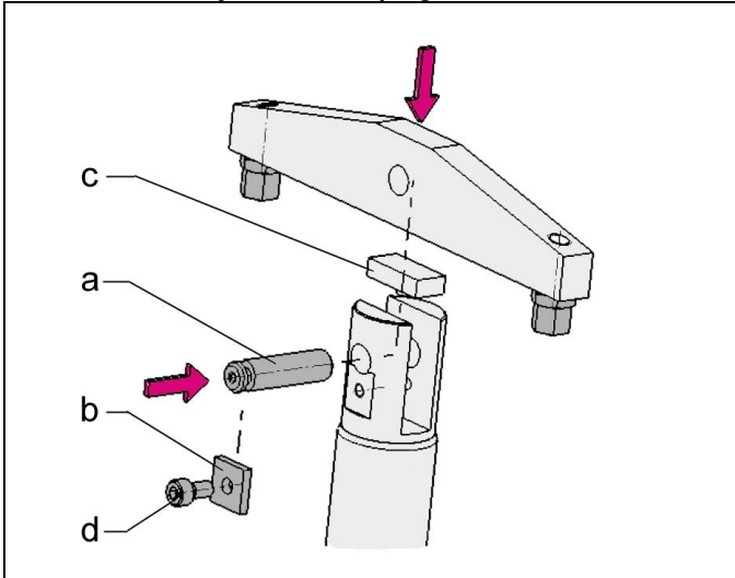
Figure 8: Assembly and disassembly of the pendulum clamping arm
