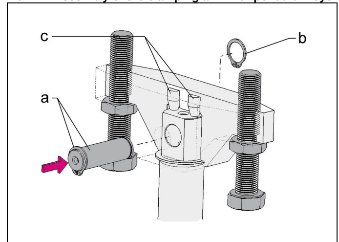
Figure 7: Assembly and disassembly of the pendulum clamping arm
