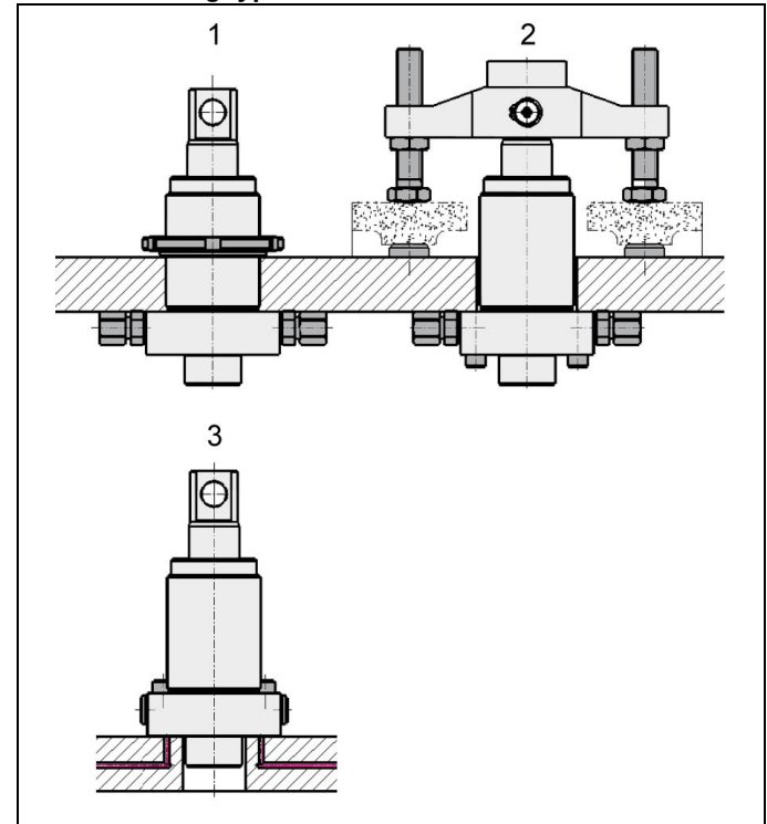
Figure 4: Mounting types
