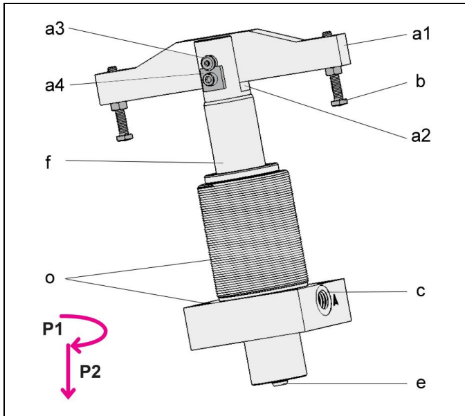
Figure 2: Components, fork head (max. 160 bar)
