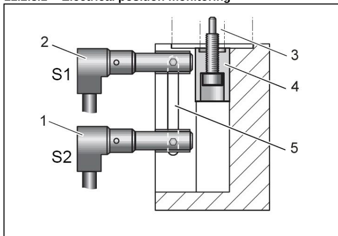
Figure 12: Design of the electrical position monitoring
