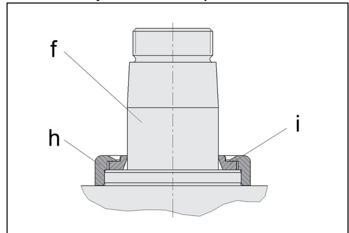
Figure 10: Metallic wiper
