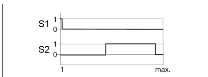
Figure 14: Signal course - unclamping
