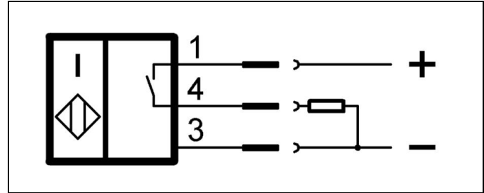
Fig. 11: Circuit diagram for pnp (+) inductive sensors
