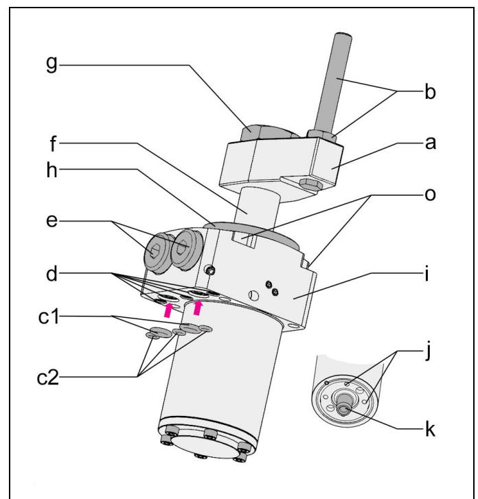
Fig. 1: Components
