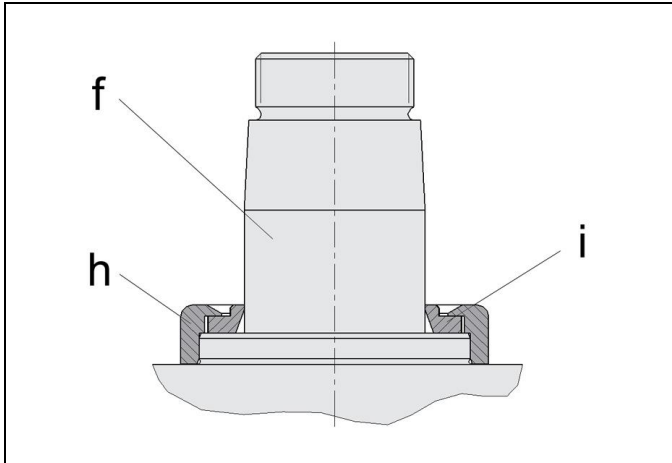
Figure 7: Metallic wiper
