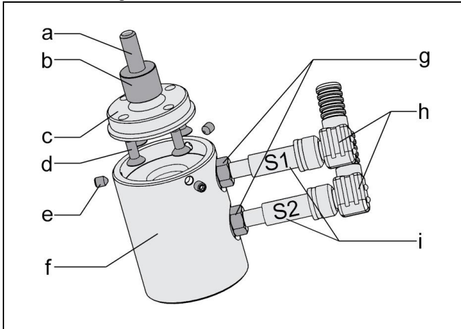
Fig. 10: Design of the electrical position monitoring
