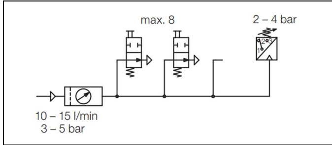
Fig. 9: Pneumatic circuit diagram
