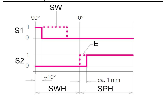
Fig. 12: Signal curve of clamping and unclamping process
