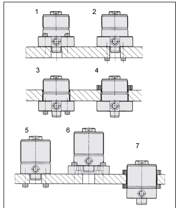
Figure 2: Fixing possibilities
