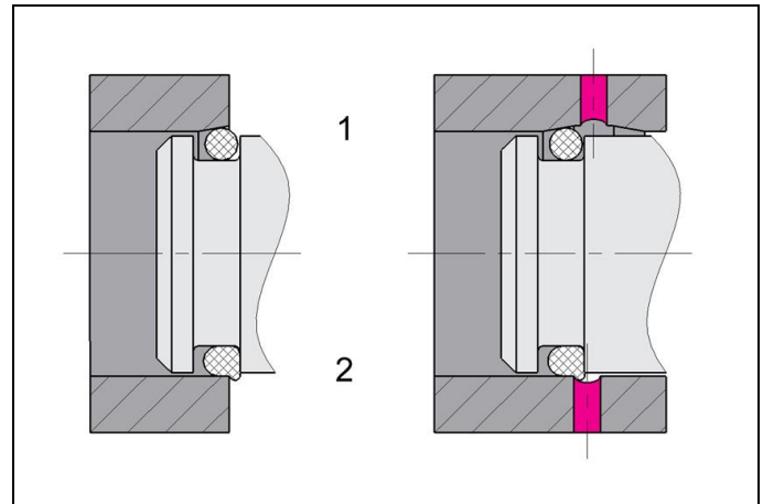
Figure 6: Installation with insertion chamfer and cross hole
