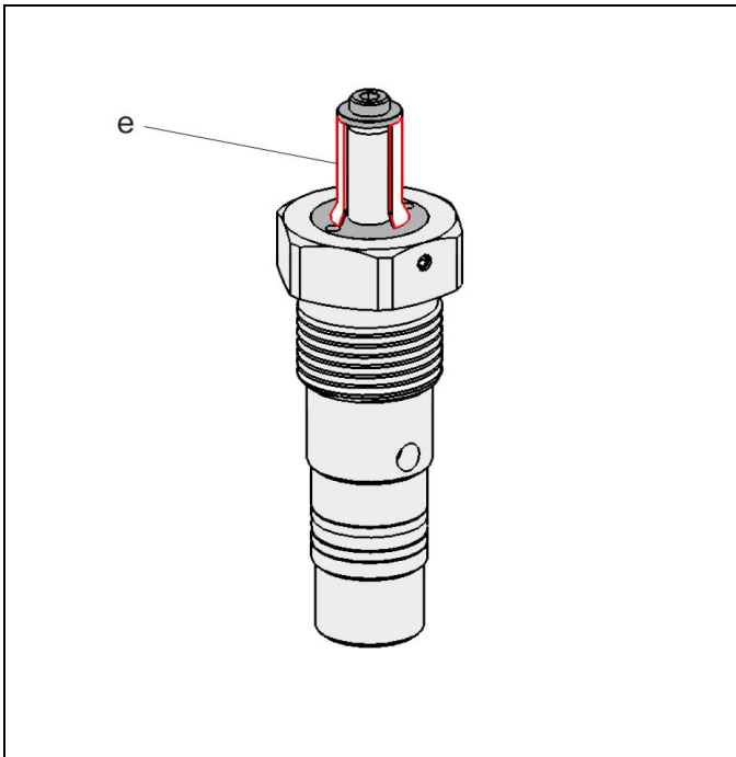
Figure 1: Swing clamp with transport safety device
