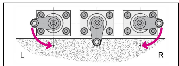
Figure 3: Swing direction
