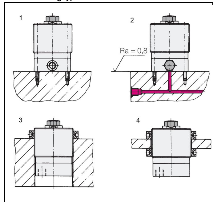
Figure 2: Fixing possibilities
