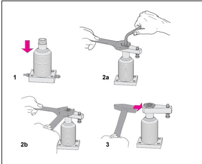
Figure 8: Assembly / disassembly (example)
