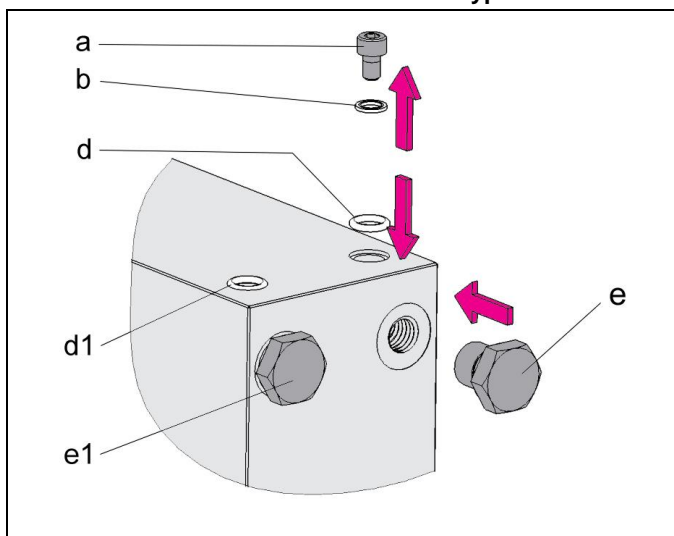
Figure 7: Example of the preparation for hydraulic ports without pipes
