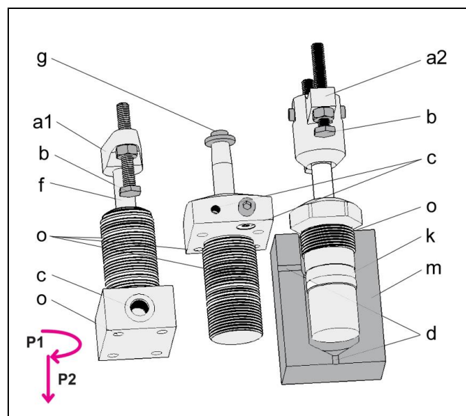
Figure 1: Components
