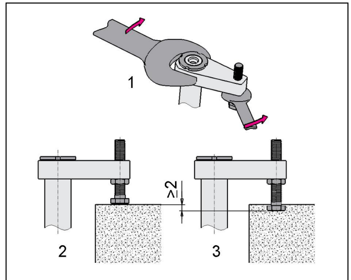
Figure 9: Adjustment of the clamping arm (example)
