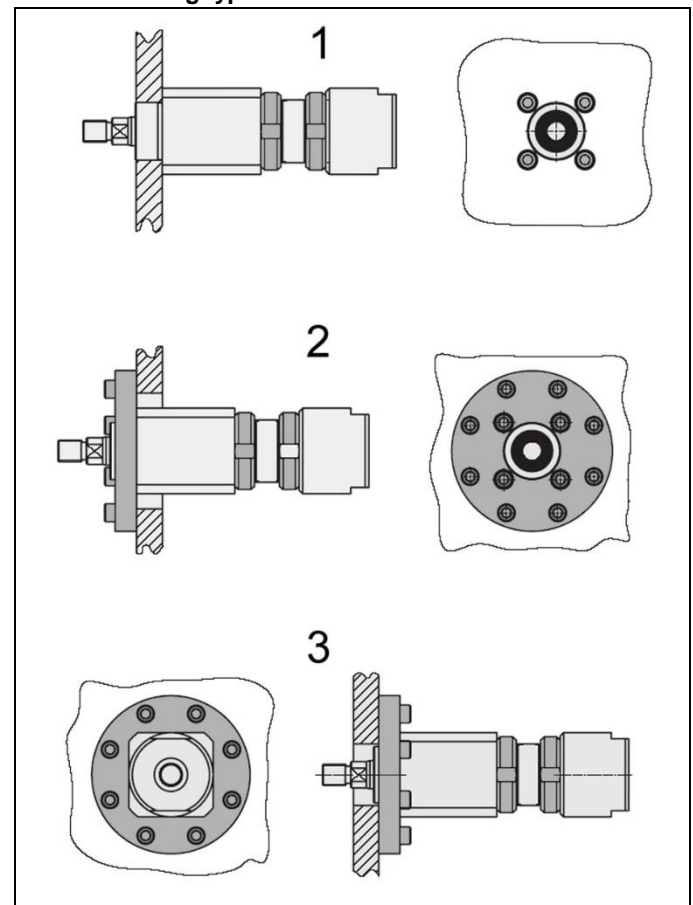
Figure 2: Fixing possibilities
