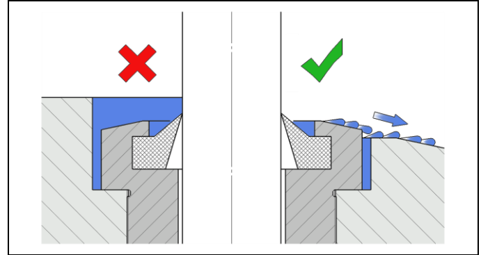
Figure 7: Discharge of coolants, using the example of a screw-in element
