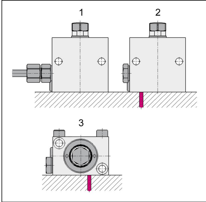
Figure 2: Fixing possibilities
