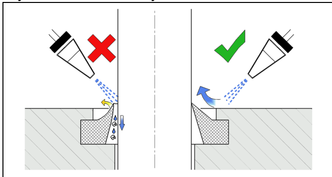
Figure 6: Swarf entry by direct coolant jet
