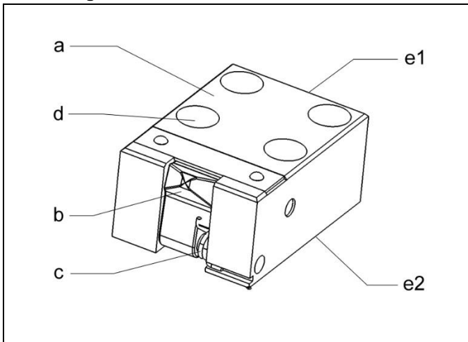
Abb. 1: Components
