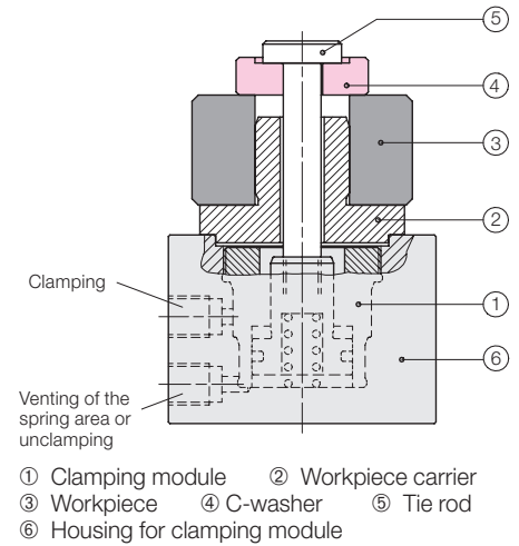
Figure 1 - Clamping with C-washer
