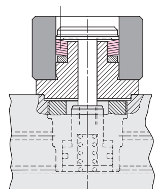
Figure 3 - Clamping with disk
