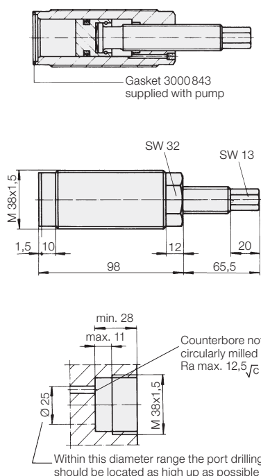
Threaded-body type
