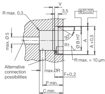
Manifold-mounting hole
