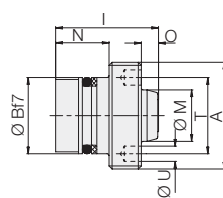
Threaded nipple
