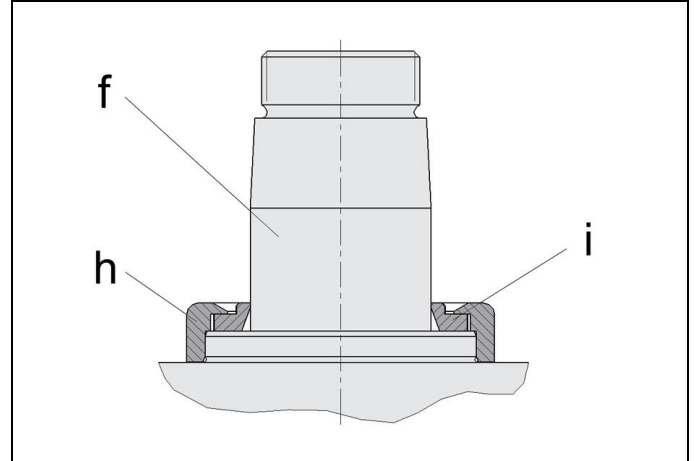
Figure 9: Metallic wiper
