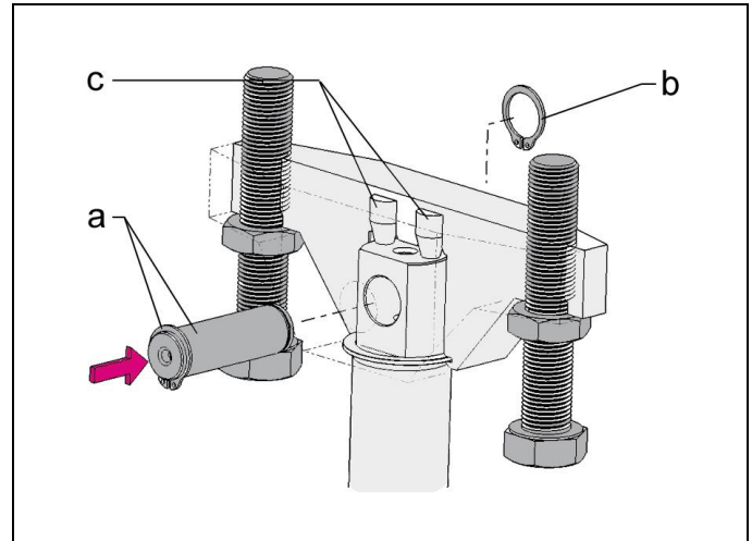
Figure 6: Assembly and disassembly of the pendulum clamping arm
