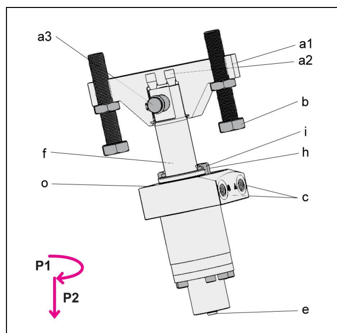
Figure 1: Components, pendulum eye (max . 500 bar)
