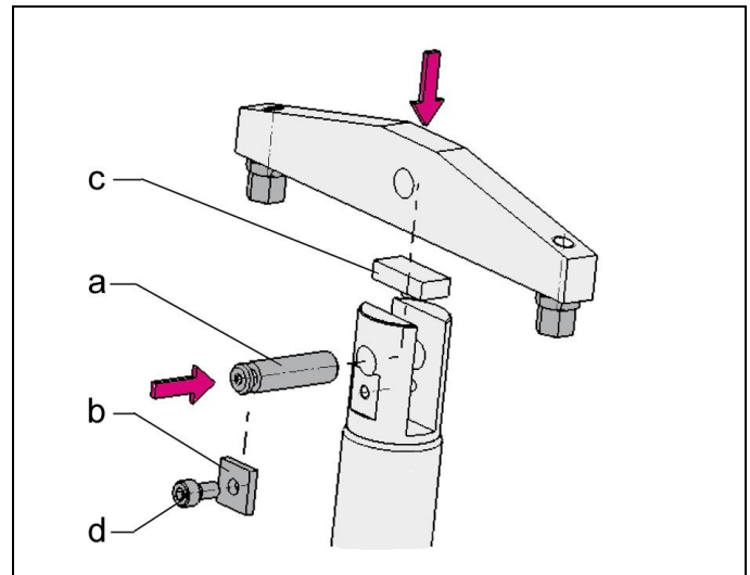
Figure 7: Assembly and disassembly of the pendulum clamping arm
